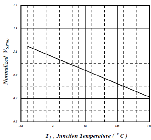
Figure 7. Gate Threshold Voltage vs Junction Temperature
